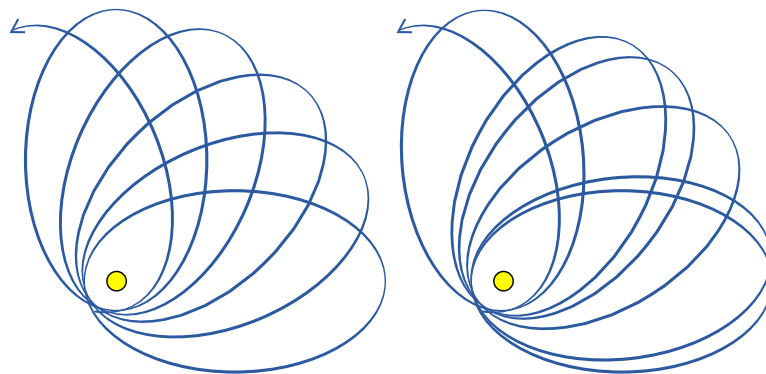
Fig. 6 An idealized uniform perihelion shift of Mercury in the direction of circulation is shown on the left. For clarity, a very high artificial eccentricity e = 0.8 is chosen. On the right is schematically depicted an irregular perihelion shift caused by the gravitational tug of other planets.
