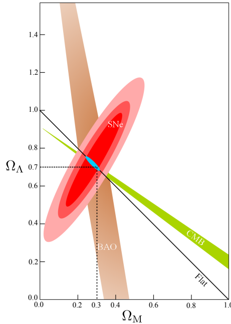
Fig. 4 Admissible values of cosmological parameters, obtained by three different methods: BAO, CMB, and SNe, intersect in a small region containing cosmological parameters \Omega_M \approx 0.3 and \Omega_\Lambda \approx 0.7 .
