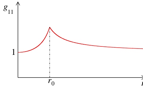
Fig. 1 The behavior of the non-differentiable component g_{11} = g_{11}(r) of the metric tensor from Eq. (10) and (13). The first derivative (\partial g_{11}/\partial r)(r_0) is not defined. The piecewise rational function g_{11} cannot be smoothed near r_0 , since then Einstein's equations (1) would not be valid in a close neighborhood of r_0 .
