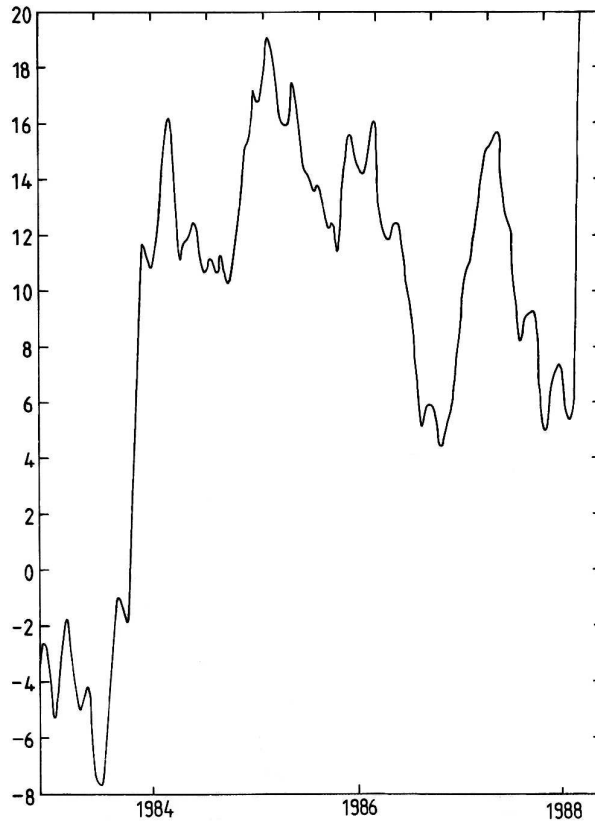
Fig. 7 The shift of the line of apsides of Mercury's orbit during five years only, calculated numerically from the N -body problem in heliocentric coordinates (adapted from [53]). The graph resembles deterministic chaos. The scale on the horizontal axis is given in years, and on the vertical axis the shift angle is in arc seconds.
