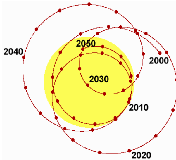
Fig. 8 The trajectory of the Newtonian center of gravity of the Solar system for the period 2000–2050. The center of the Sun (whose diameter is almost 1.4 million km) is at the origin of the heliocentric system. The center of gravity shifts each day by about 1000 km, while the additional relativistic perihelion shift of Mercury is by Eq. (36) on average of only 96 km in a year.
