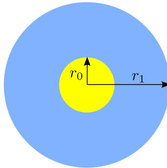
Fig. 2 A schematic illustration of the Sun with its spherically symmetric neighborhood.
