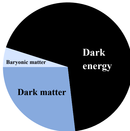
Fig. 3 Results of the Planck satellite [52] are interpreted in such a way that our universe consists of about 6 times more dark matter than ordinary baryonic matter. However, they are based on the normalized Friedmann equation (23), which was derived using excessive extrapolations by many orders of magnitude.
