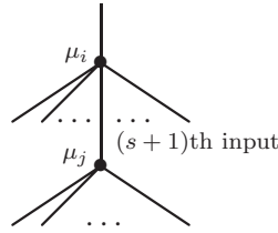
FIGURE 2. The graph corresponding to \mu_i \circ_{s+1} \mu_j .
