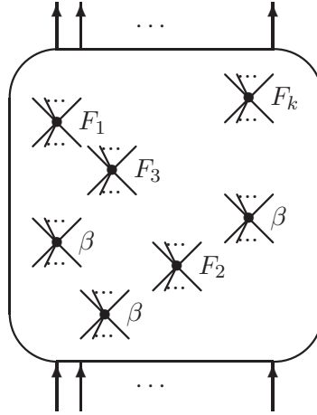
FIGURE 1. \text{End}_T^{\mathfrak{C}} -decorated graph \Gamma_{\{\beta\}}^{\{v_1, \dots, v_k\}}[F_1, \dots, F_k] . Vertices labelled F_i are decorated by F_i(e_{v_i}) , 1 \leq i \leq k , the remaining vertices are decorated by \beta(e_v) .
