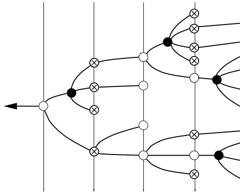
Fig. 9. The w -image of the tree \beta \in \text{LTr} from Fig. 2.
