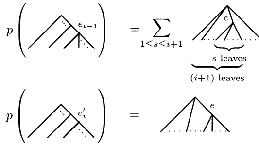
FIGURE 7. Each of the trees labeling the faces of K_n appears precisely once as a term in \partial\bar{b}(n) . The orientation elements (not shown in the figure) are (-1)^{i-1}e_1 \wedge \cdots \wedge \hat{e}_i \wedge \cdots \wedge e_{n-2} in the upper left, (-1)^i e_1 \wedge \cdots \wedge \hat{e}_i \wedge \cdots \wedge e_{n-2} in the lower left, and e for both trees on the right.
