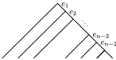
FIGURE 2. The maximal binary tree \bar{b}(n) .
